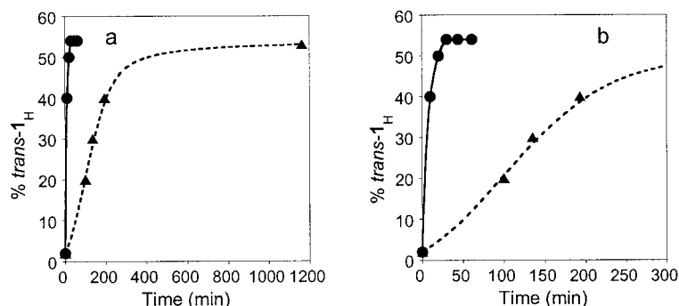
Figure 1. a) (— and solid circles): percentage of trans - 1 H formed in the reaction of cis - 1 H (40 mM) with the Pd 0 complex generated from Pd 0 (PPh 3 ) 4 (20 mM) in CDCl 3 at 25 °C, as determined by 1 H NMR spectroscopy. (--- and solid triangles): percentage of trans - 1 H formed in the reaction of cis - 1 H (40 mM) with the Pd 0 complex generated from Pd 0 (dba) 2 (20 mM) and PPh 3 (40 mM) in CDCl 3 at 25 °C. b) Same data as in Figure 1 (a) from 0 to 300 min.
