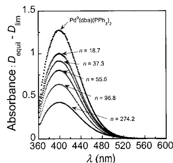
Figure 3. UV spectrum of a solution of Pd(dba) 2 (1 mM) and PPh 3 (2 mM) in the presence of n equiv. of cis -1 H at 25 °C. D_{\text{equil}} = absorbance of Pd(dba)(PPh 3 ) 2 at equilibrium in the presence of n equiv. of cis -1 H ; D_{\text{lim}} = residual absorbance observed after addition of PhI (5 mM).
