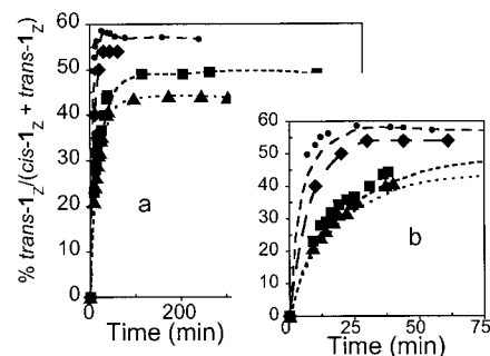
Figure 5. Percentage of trans - 1 Z formed in the reaction of cis - 1 Z (40 mM) with the Pd 0 complex generated from Pd 0 (PPh 3 ) 4 (20 mM) in CDCl 3 at 25 °C, as determined by 1 H NMR spectroscopy. (●) Z = Cl; (◆) Z = H; (■) Z = Me; (▲) Z = OMe.
