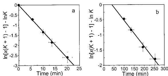
Figure 2. a) Kinetics of the isomerization of cis -1 H to trans -1 H catalyzed by the Pd 0 complex generated from Pd 0 (PPh 3 ) 4 (20 mM) in CDCl 3 at 25 °C. Plot of \ln[x(K+1)-1] - \ln K against time; x = [cis-1_Z]/C_0 at t , C_0 = initial concentration of cis -1 H = 40 mM, K = equilibrium constant between cis -1 H and trans -1 H determined from the data in part a of Figure 1. b) Same as in part a of Figure 2 for the kinetics of isomerization cis -1 H ( C_0 = 40 mM) to trans -1 H catalyzed by the Pd 0 complex generated from Pd 0 (dba) 2 (20 mM) and PPh 3 (40 mM) in CDCl 3 at 25 °C.
