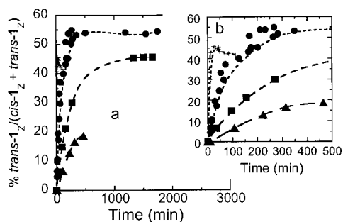
Figure 4. Percentage of trans - 1 Z formed in the reaction of cis - 1 Z (40 mM) with the Pd 0 complex generated from Pd 0 (dba) 2 (20 mM) and PPh 3 (40 mM) in CDCl 3 at 25 °C, as determined by 1 H NMR spectroscopy. (+) Z = NO 2 ; (●) Z = Cl; (■) Z = Me; (▲) Z = OMe.
