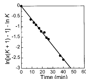
Figure 6. a) Kinetics of the isomerization cis - 1 OMe to trans - 1 OMe catalyzed by the Pd 0 complex generated from Pd 0 (PPh 3 ) 4 (20 mM) in CDCl 3 at 25 °C. Plot of \ln[x(K+1)-1] - \ln K against time ( x = [cis-1_{OMe}]/C_0 at t , C_0 = initial concentration of cis - 1 OMe = 40 mM, K = equilibrium constant between cis - 1 OMe and trans - 1 OMe ).
